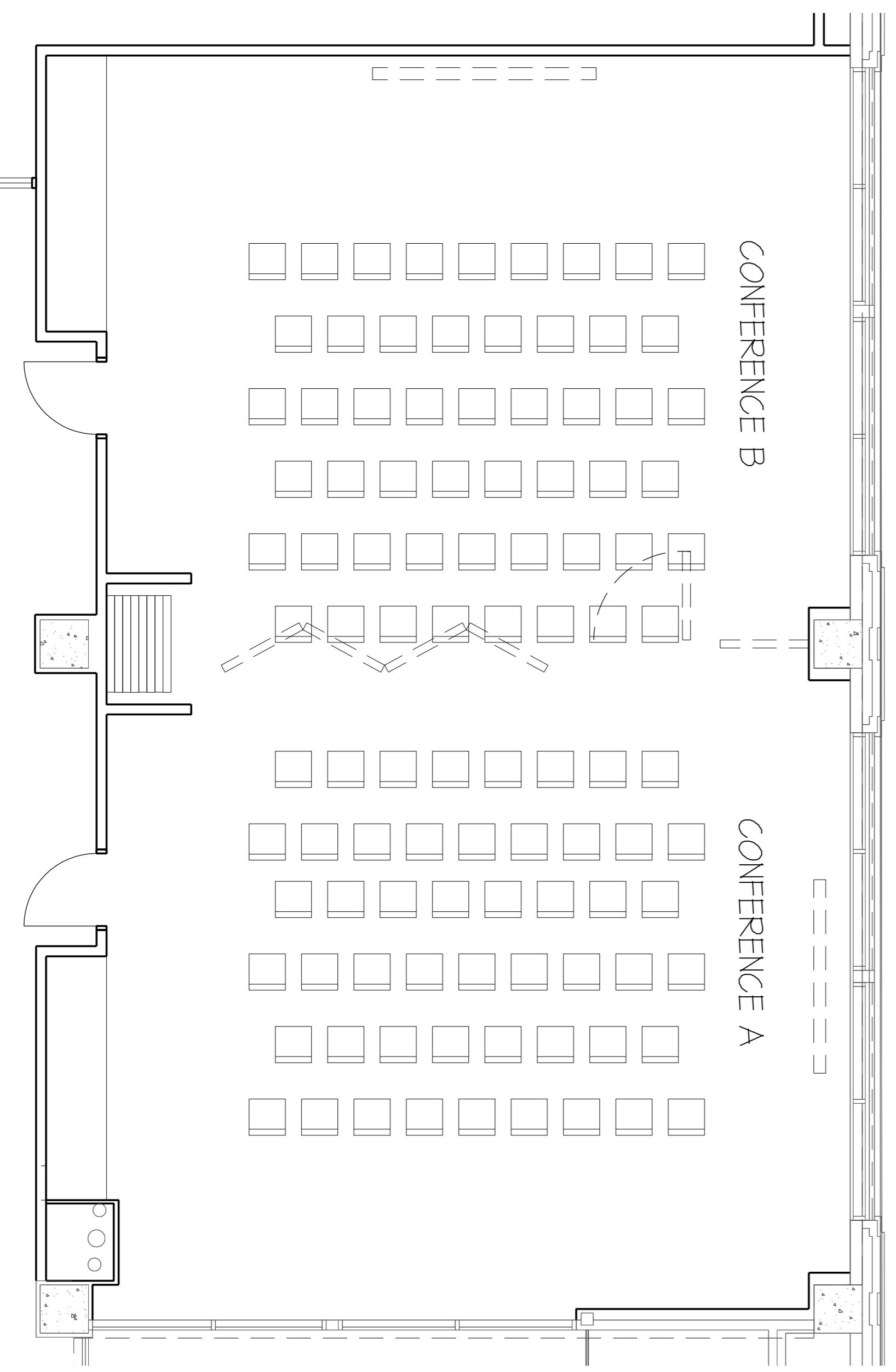
CONFERENCE CTR FURNITURE LAYOUT - C
